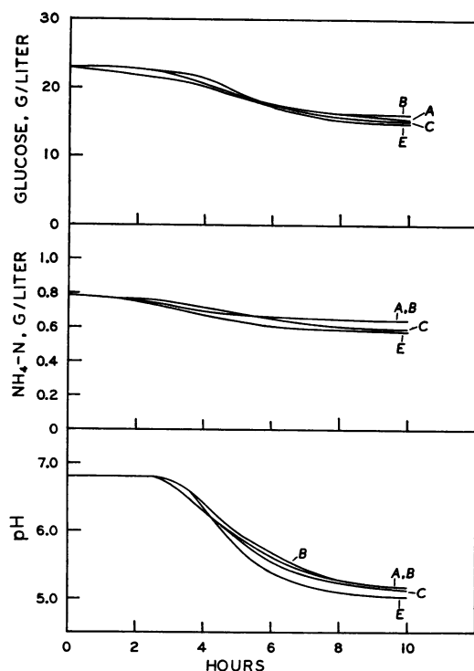
FIG. 8. Glucose utilization, \text{NH}_4\text{-N} utilization, and pH curves at OAR 0.16. Symbols same as Fig. 1.
