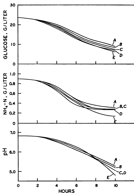
FIG. 5. Glucose utilization, \text{NH}_4\text{-N} utilization, and pH curves at OAR 2.5. Symbols same as Fig. 1.
