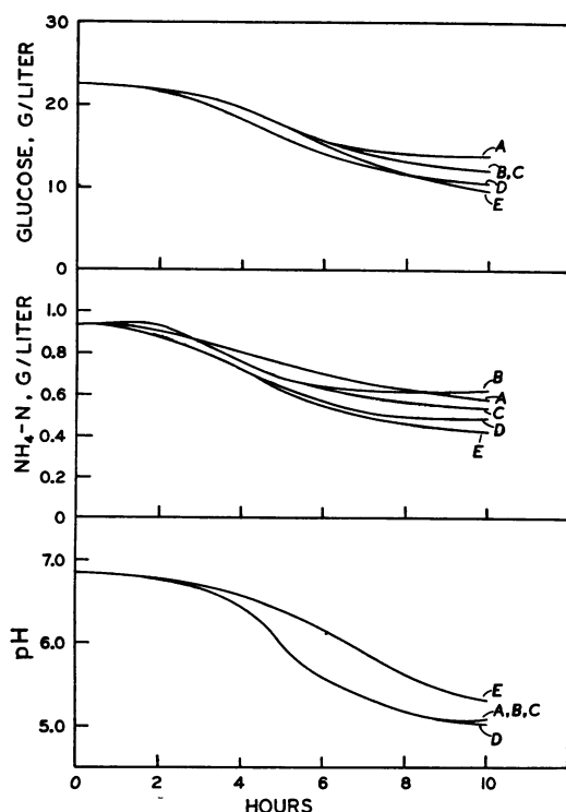
FIG. 7. Glucose utilization, \text{NH}_4\text{-N} utilization, and pH curves at OAR 0.65. Symbols same as Fig. 1.
