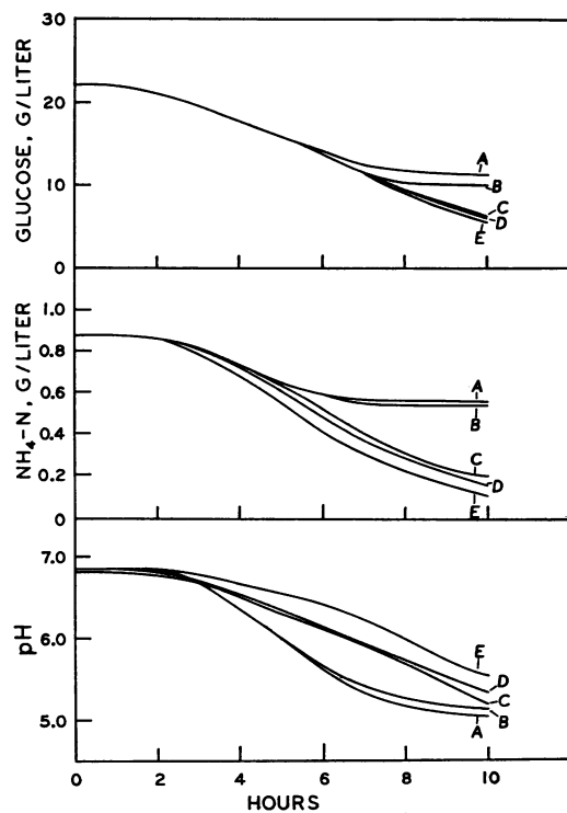
FIG. 6. Glucose utilization, \text{NH}_4\text{-N} utilization, and pH curves at OAR 1.0. Symbols same as Fig. 1.
