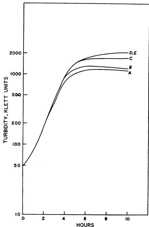
FIG. 3. Fermentor and shake-flask growth curves at OAR 0.65. Symbols same as Fig. 1.
