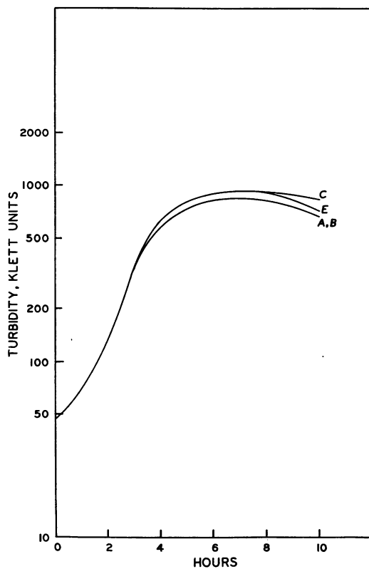
FIG. 4. Fermentor and shake-flask growth curves at OAR 0.16. Symbols same as Fig. 1.
